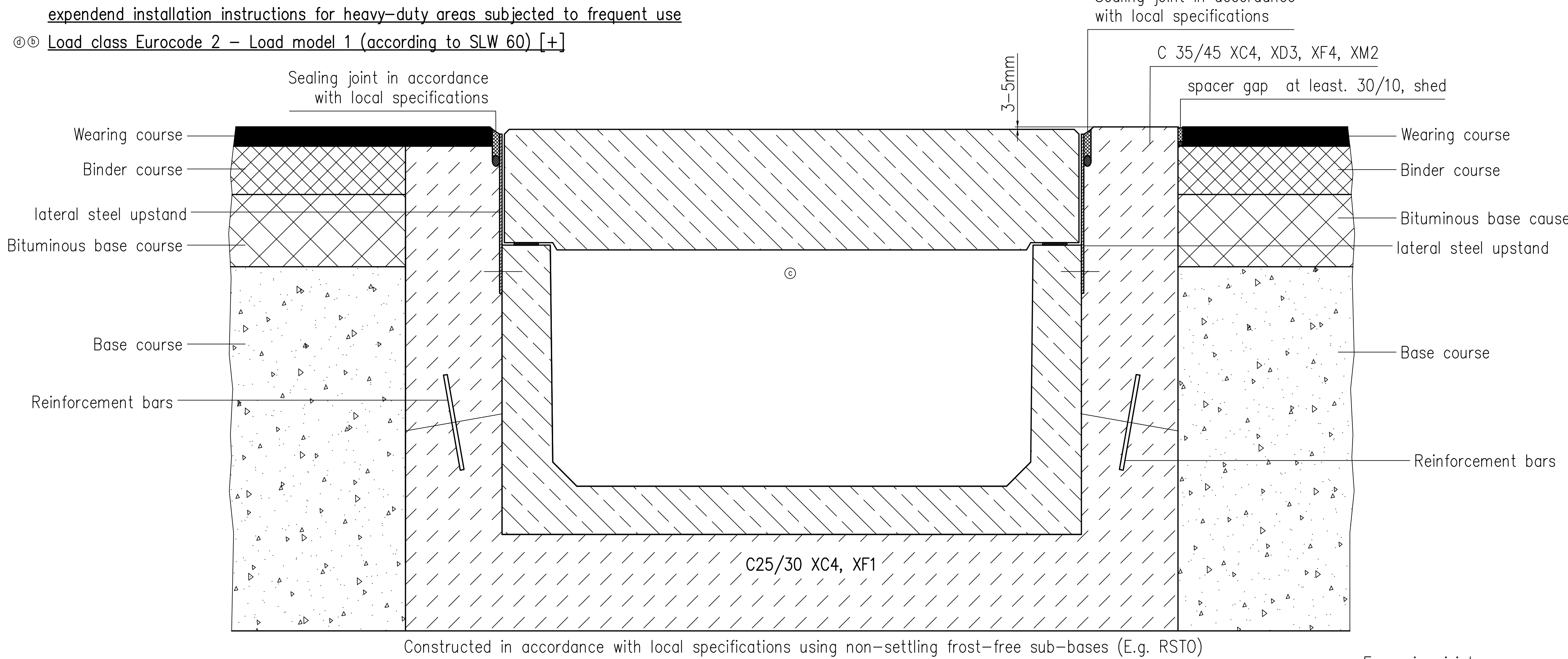
Constructed in accordance with local specifications using non-settling frost-free sub-bases (E.g. RSTO)
